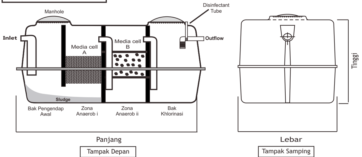
Sketsa Septic Tank Fiberglass
